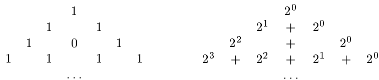
Figure 1. Rows of Pascal's triangle, reduced modulo 2 and interpreted as binary numbers.
